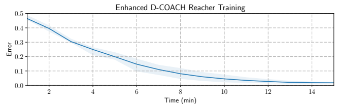
Fig. 9: Evolution of the error while learning the reacher task.
